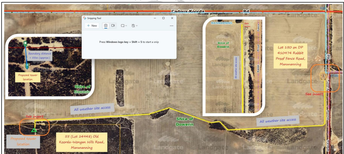
FIGURE 3 - ACCESS PLAN
